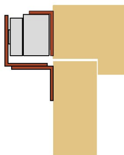
inward opening using optional Z & L bracket set
