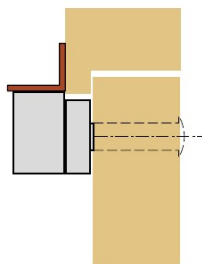
outward opening using optional L bracket
