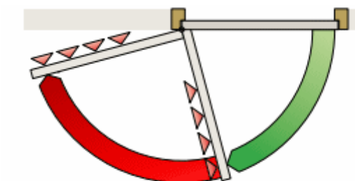
Adjustable backcheck activation zone
