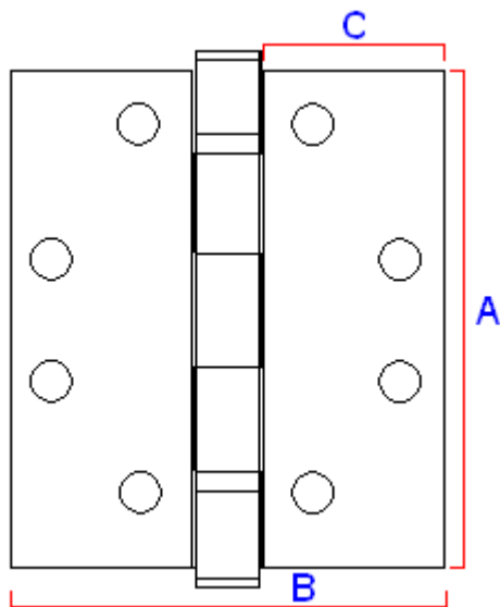
20251.1 Dimension On Diagram
