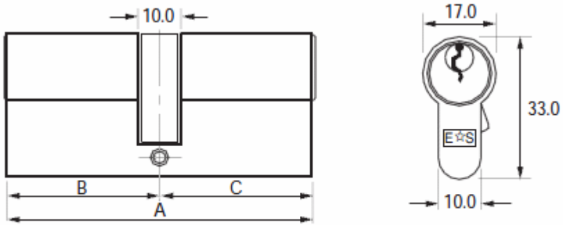
All measurements in mm
